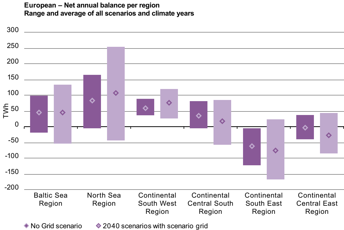
Figure 10: Net annual region balance in 2040, depending on assumed grid status
