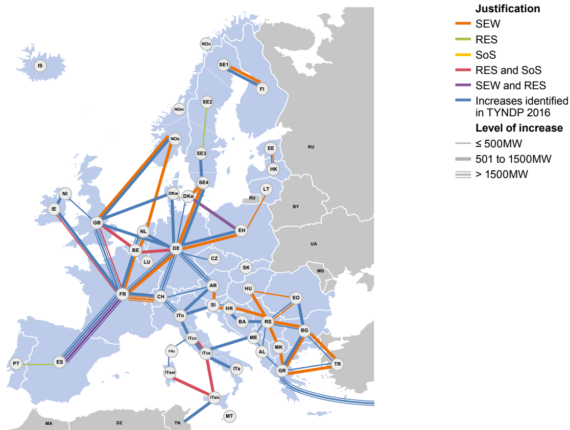
Figure 4: Justification of increases from DG2040 on top of confirmed increases from last TYNDP 3
