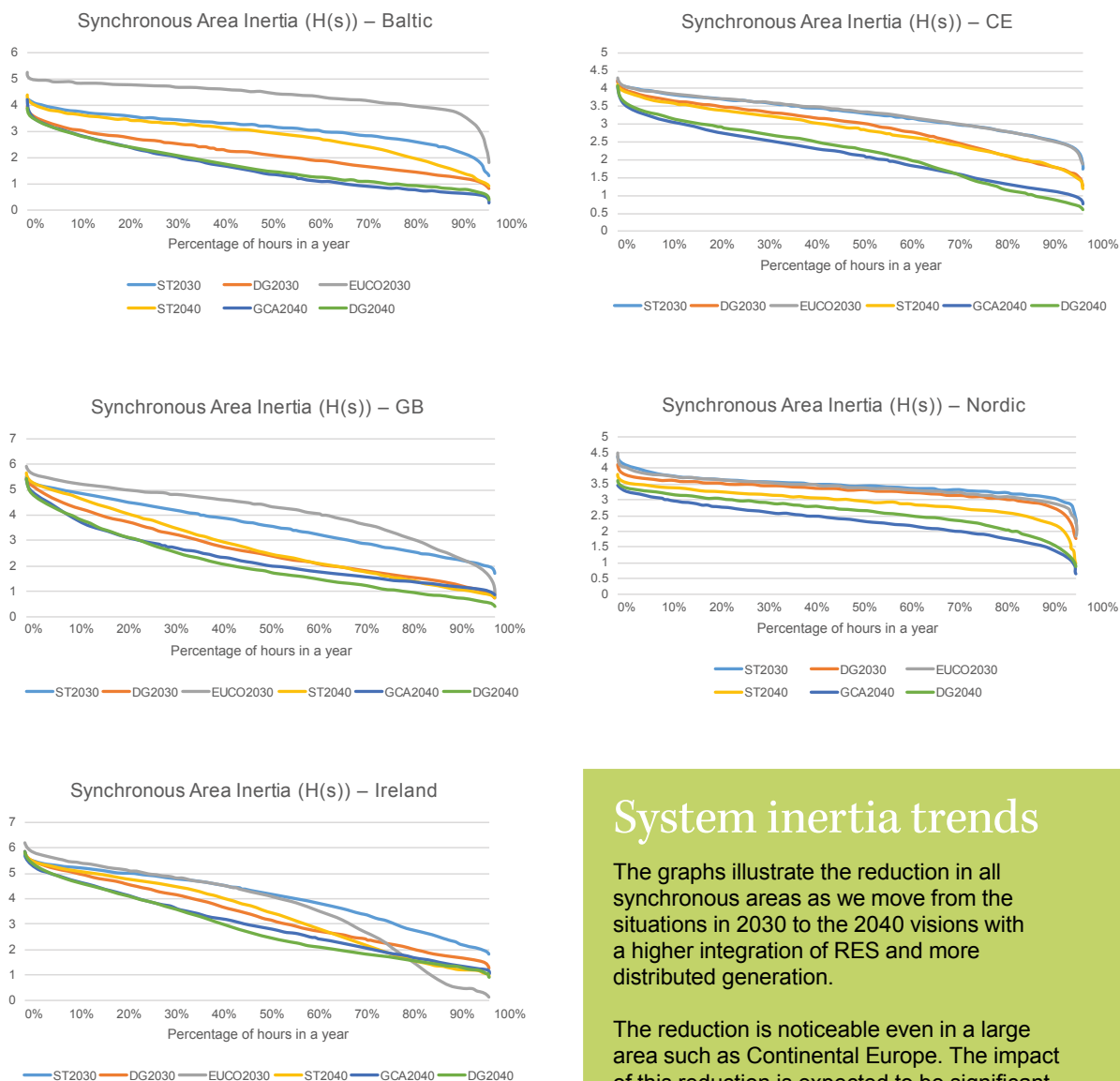
Figure 16: Duration curves of estimated synchronous areas equivalent inertia (H(s))
