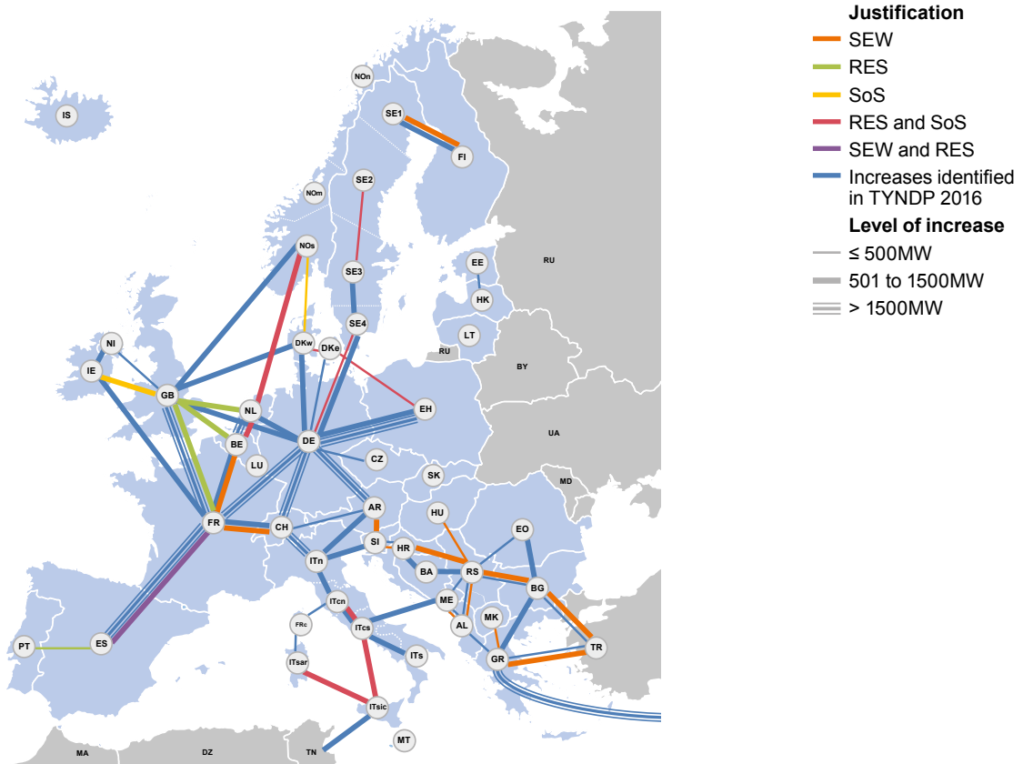
Figure 3: Justification of increases from ST2040 on top of confirmed increases from last TYNDP
