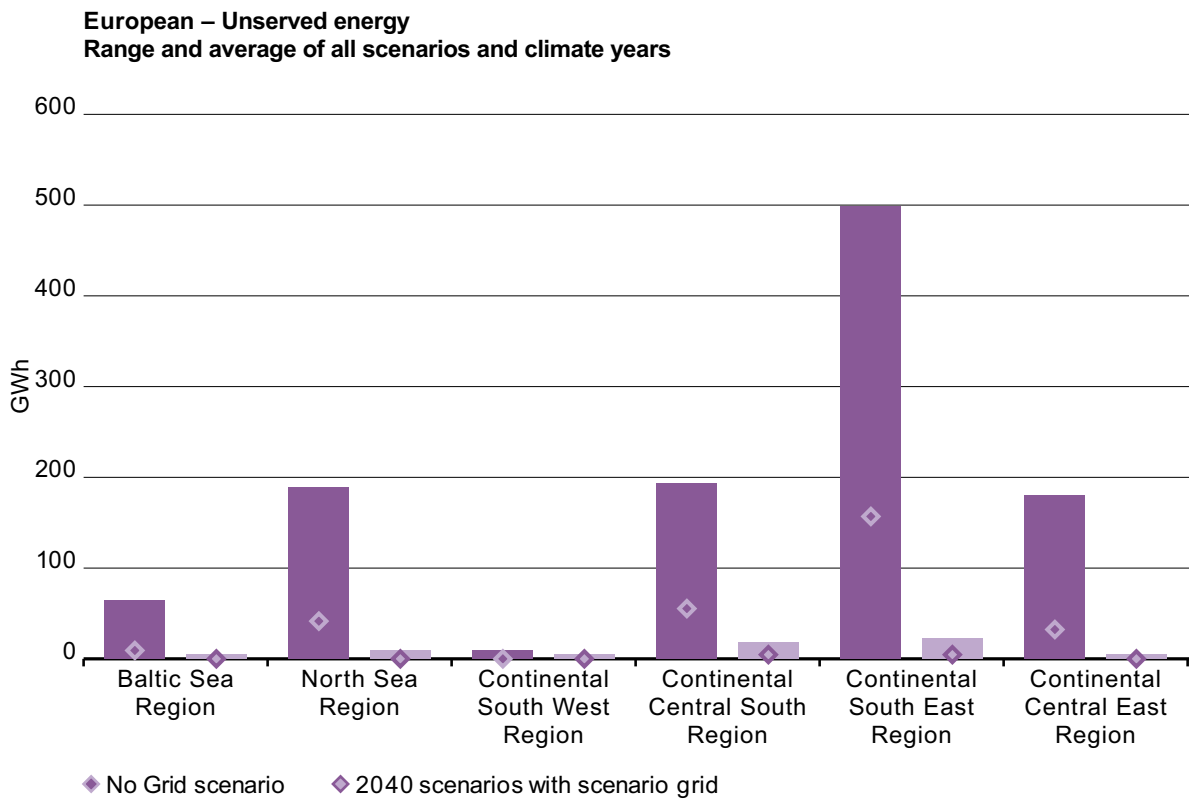
Figure 11: Unserved energy in 2040, depending on assumed grid status (absolute values in GWh)
