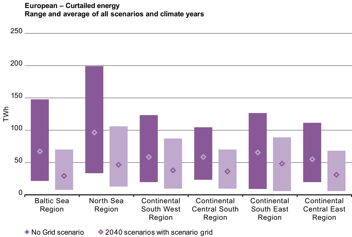
Figure 13: Curtailed energy in 2040, depending on assumed grid status
