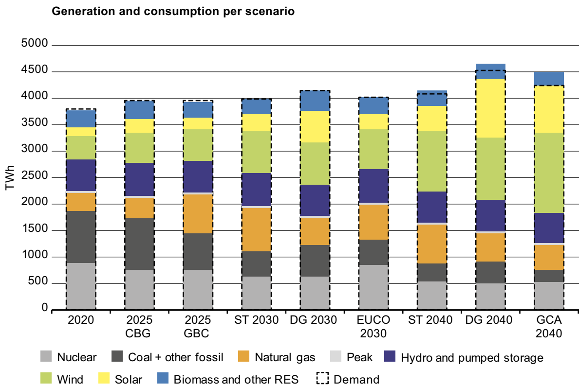
Figure 19: Electricity net generation by source and consumption per scenario
