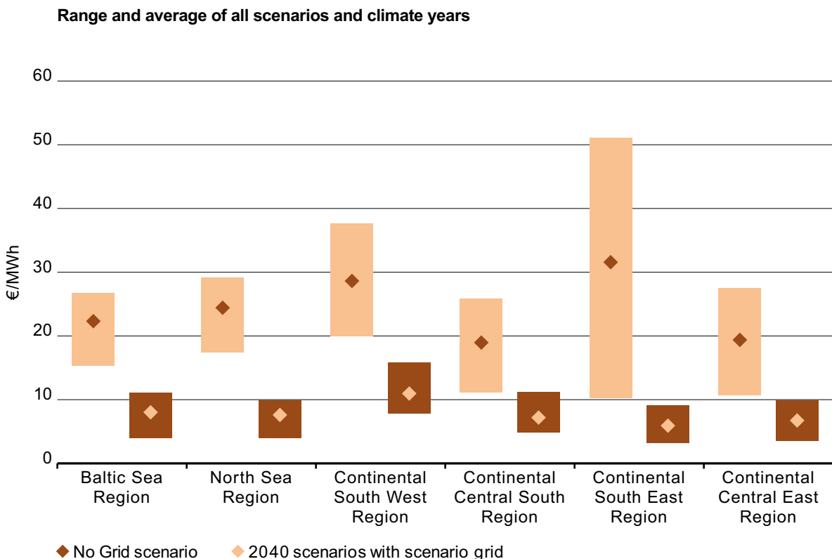
Figure 8: Range and average annual marginal cost differences
