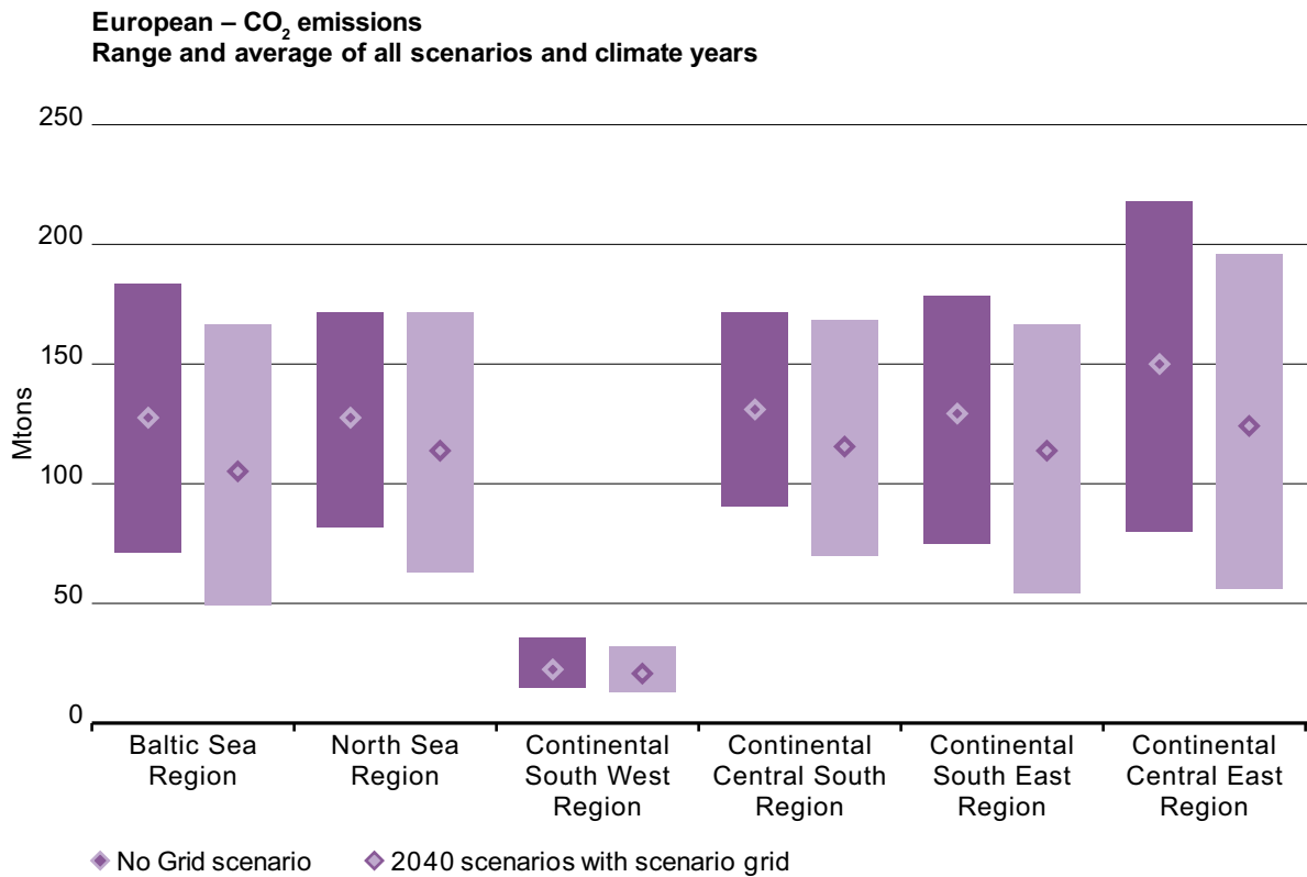
Figure 14: CO 2 emissions in 2040, depending on assumed grid status
