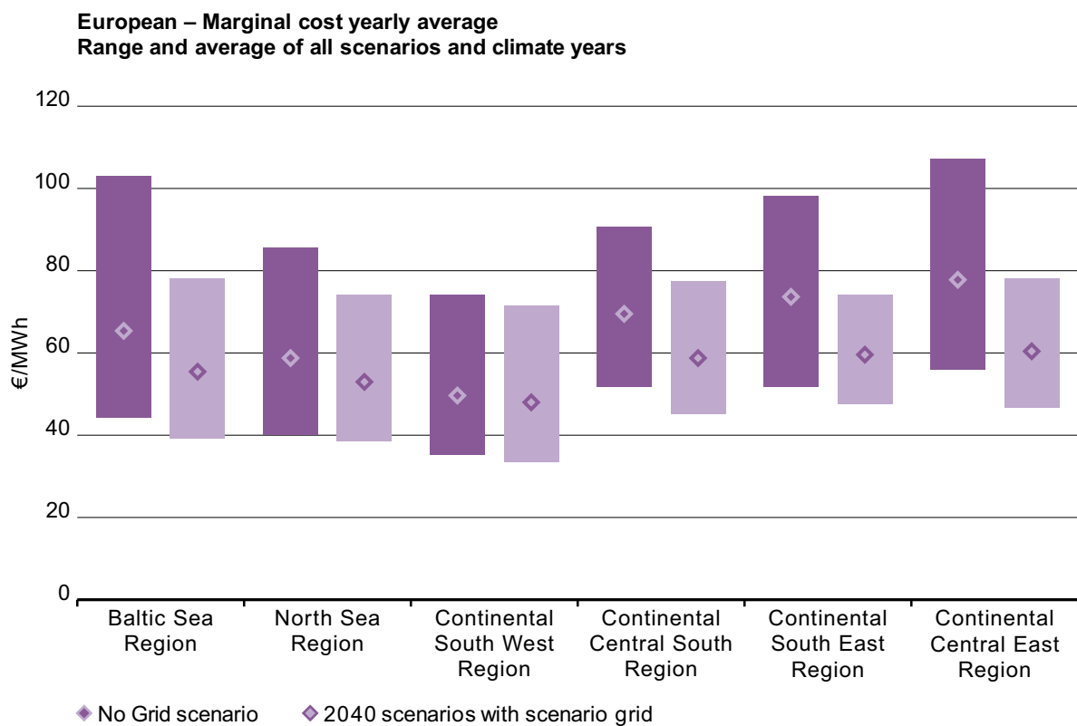
Figure 9: Range and average annual marginal cost per regional group
