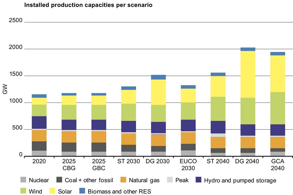
Figure 18: Electricity installed generation capacity by source and scenario
