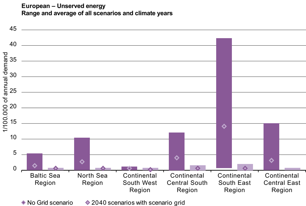
Figure 12: Unserved energy in 2040, depending on assumed grid status (in percentage of demand)
